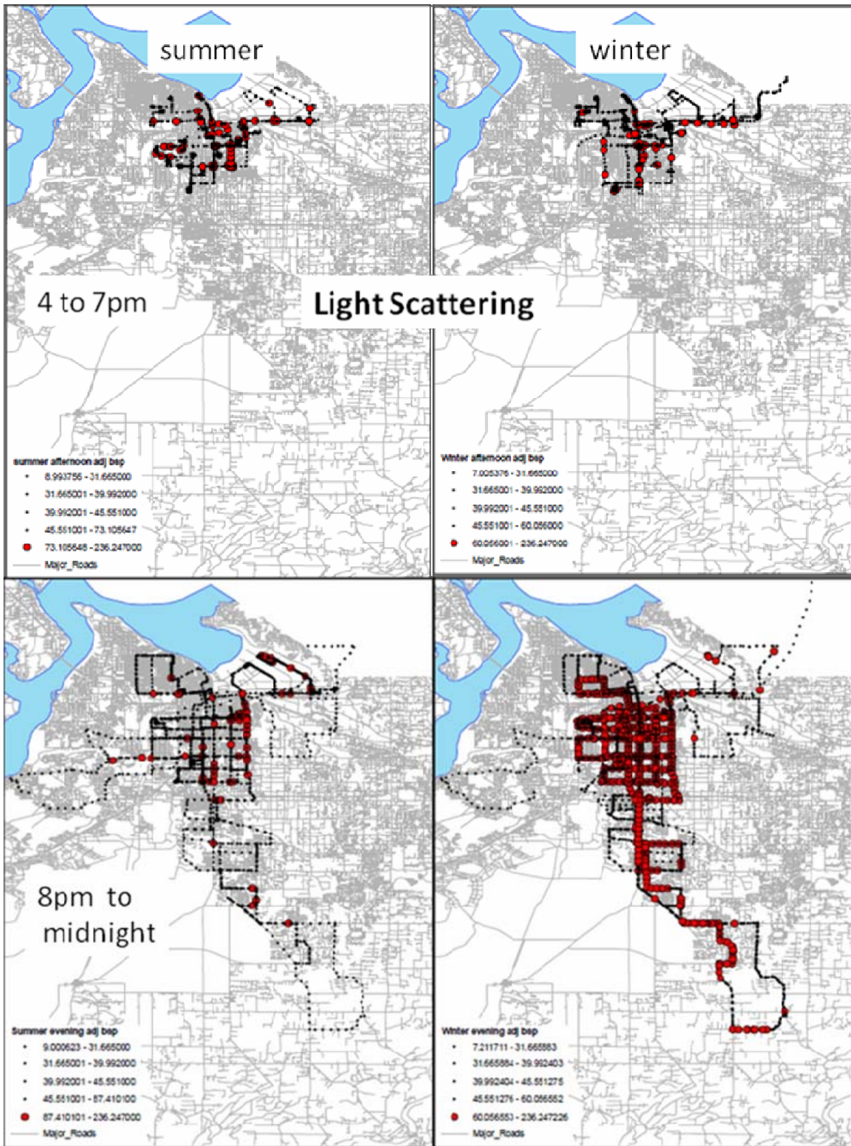
Figure 3.3.1: Spatial Distribution of Temporally Adjusted Particle Light Scattering Coefficient (measurements were taken in the late afternoon and evening on selected winter days between December 2008 and February 2009 and on selected summer days between July and August 2009)
