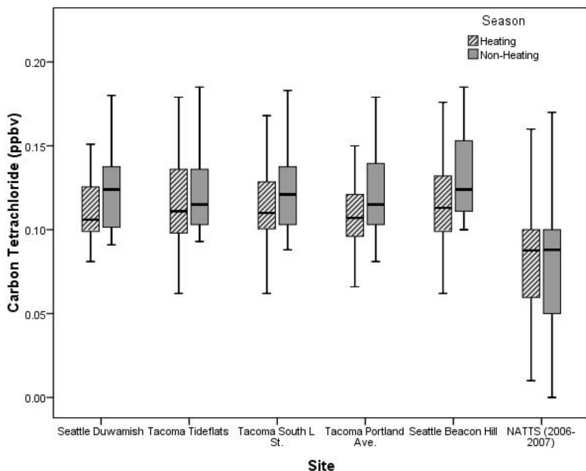
Figure 3.1.6: Box and Whisker Plots for Carbon Tetrachloride: results by site and season
