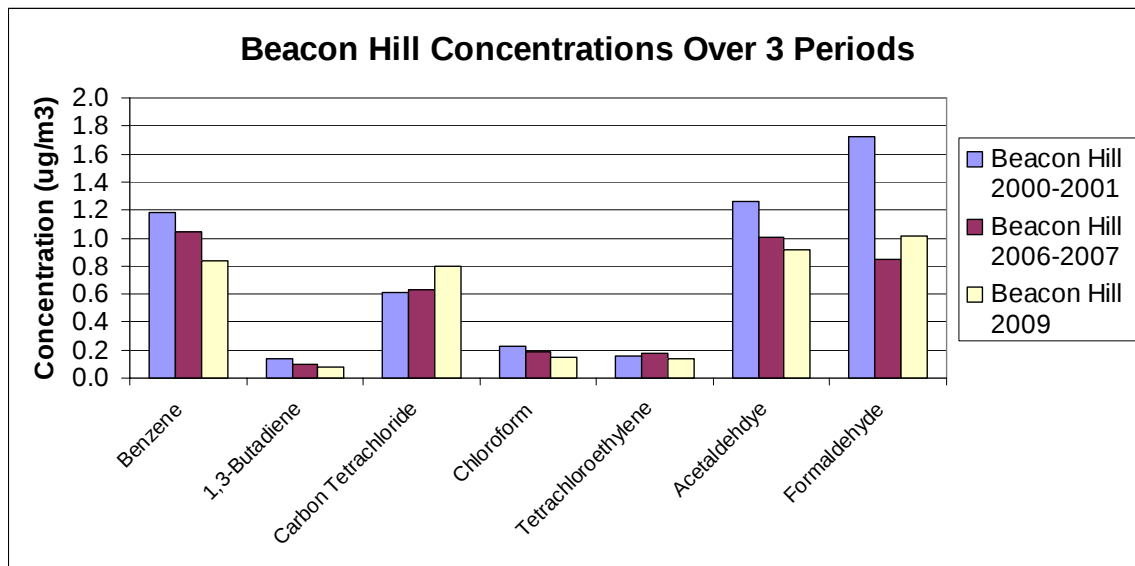
Figure 3.1.17: Beacon Hill Concentrations Over 3 Periods
