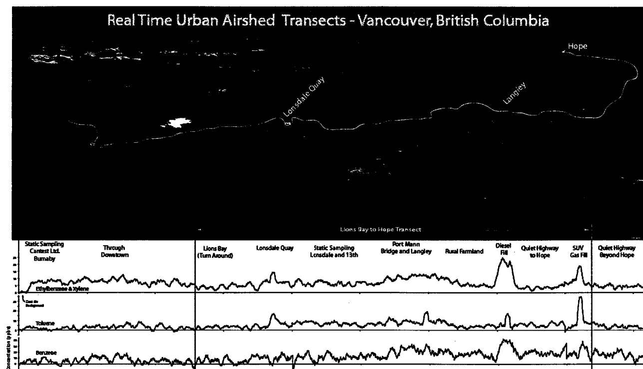
Figure 3-2. Urban Airshed Transects from British Columbia using MIMS
