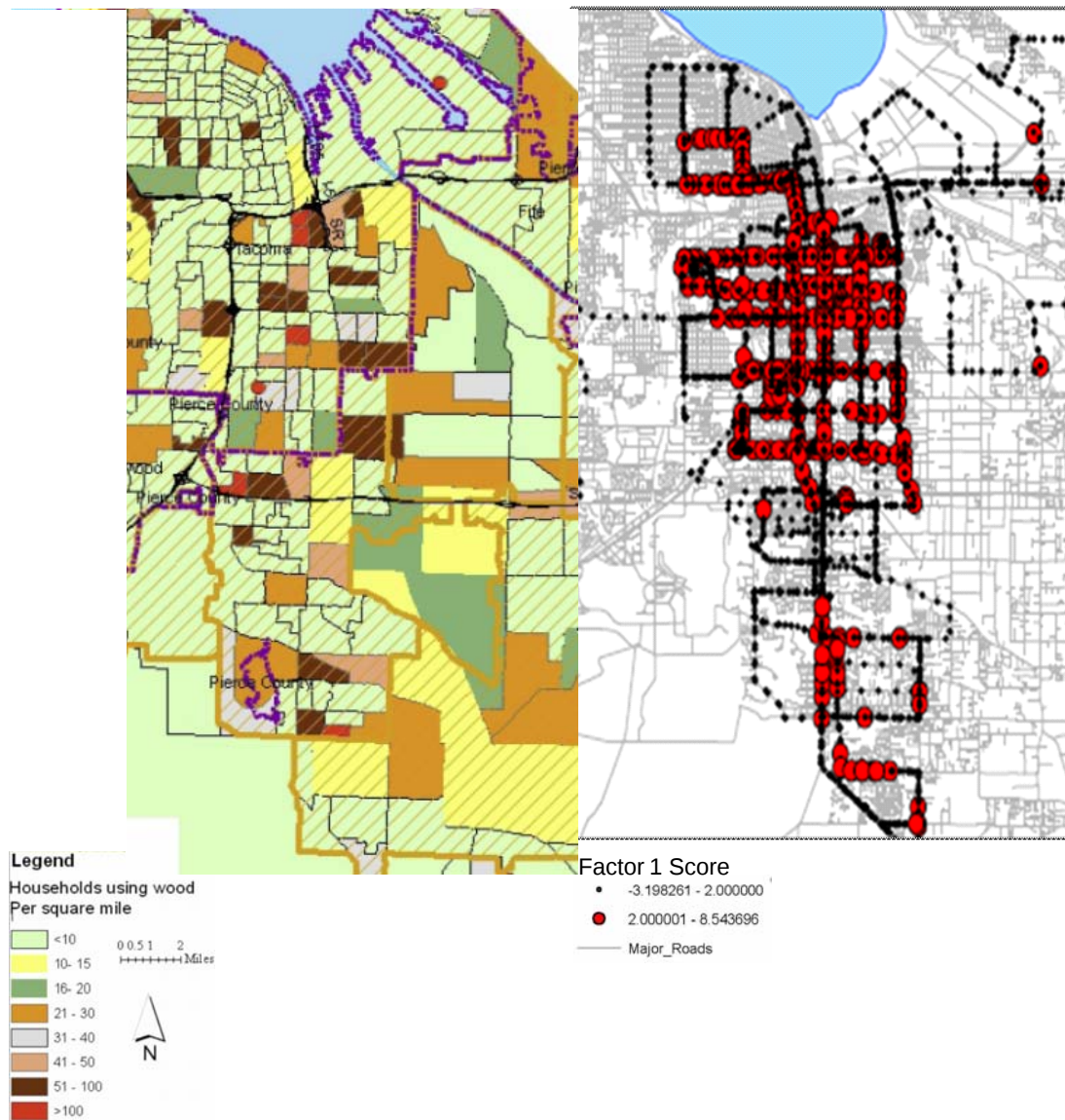
Figure 3.3.4: Spatial Distribution of Woodstove Use Survey Data versus winter, nighttime contributions from a multivariate factor derived from principal component analysis
