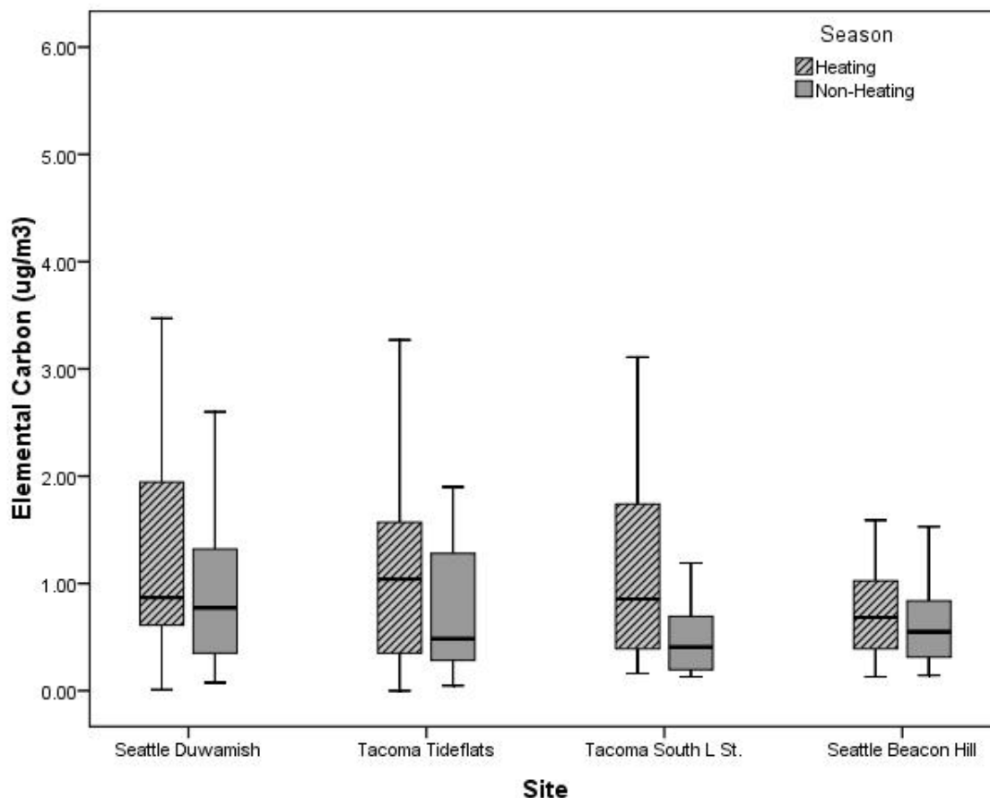
Figure 3.1.10: Box and Whisker Plots for Elemental Carbon: results by site and season
