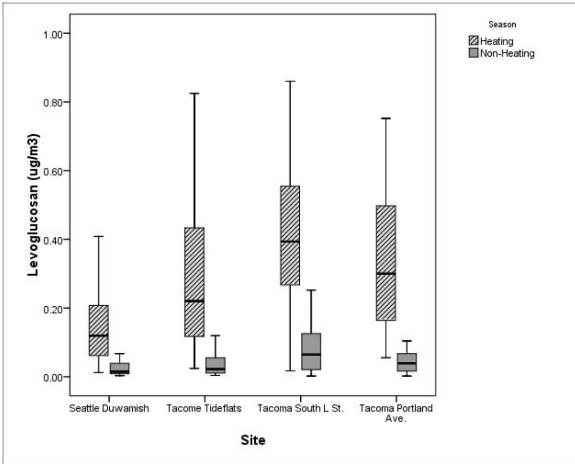
Figure 3.1.13: Box and whisker Plots for Levoglucosan: results by site and season
