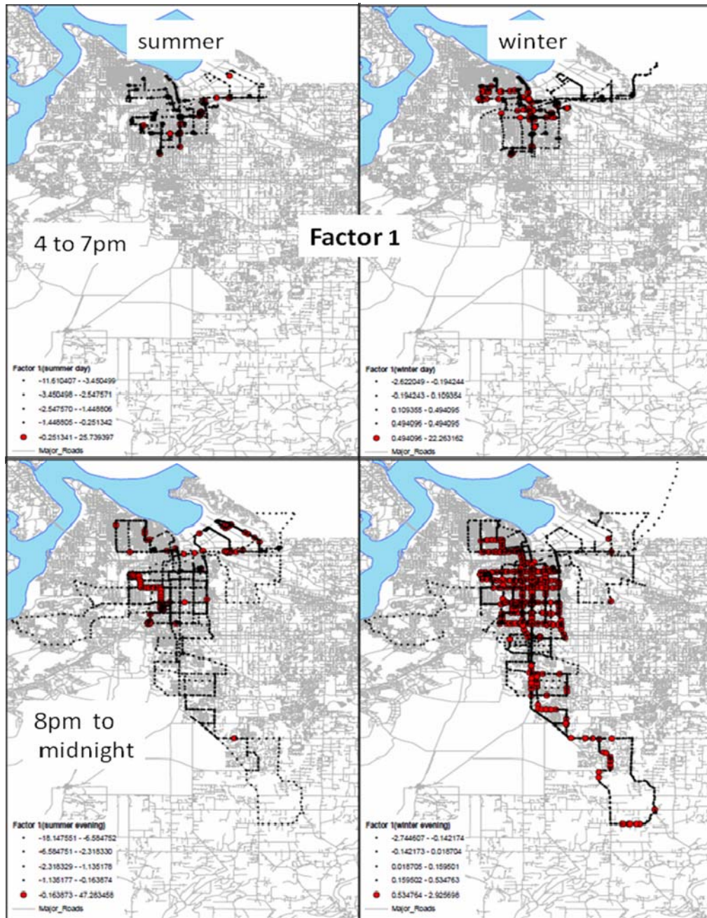
Figure D.5: Spatial distribution of Varimax Factor #1 scores.
