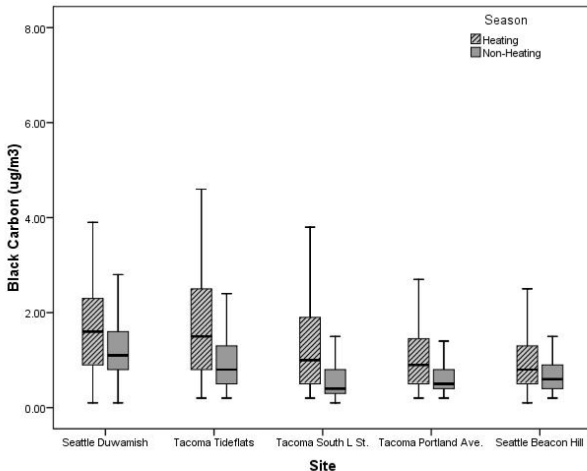
Figure 3.1.9: Box and Whisker Plots for Black Carbon: results by site and season
