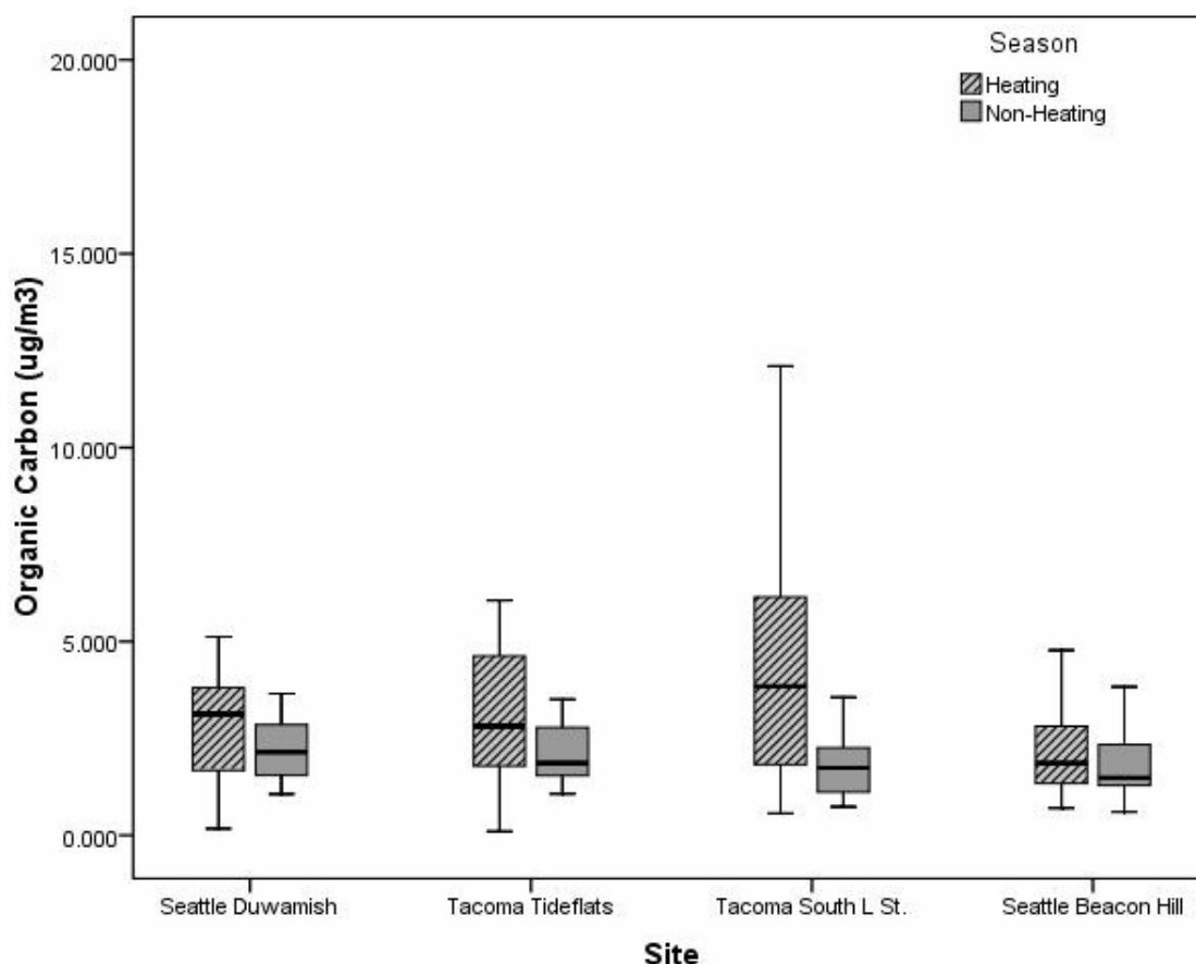
Figure 3.1.12: Box and Whisker Plots for Organic Carbon: results by site and season
