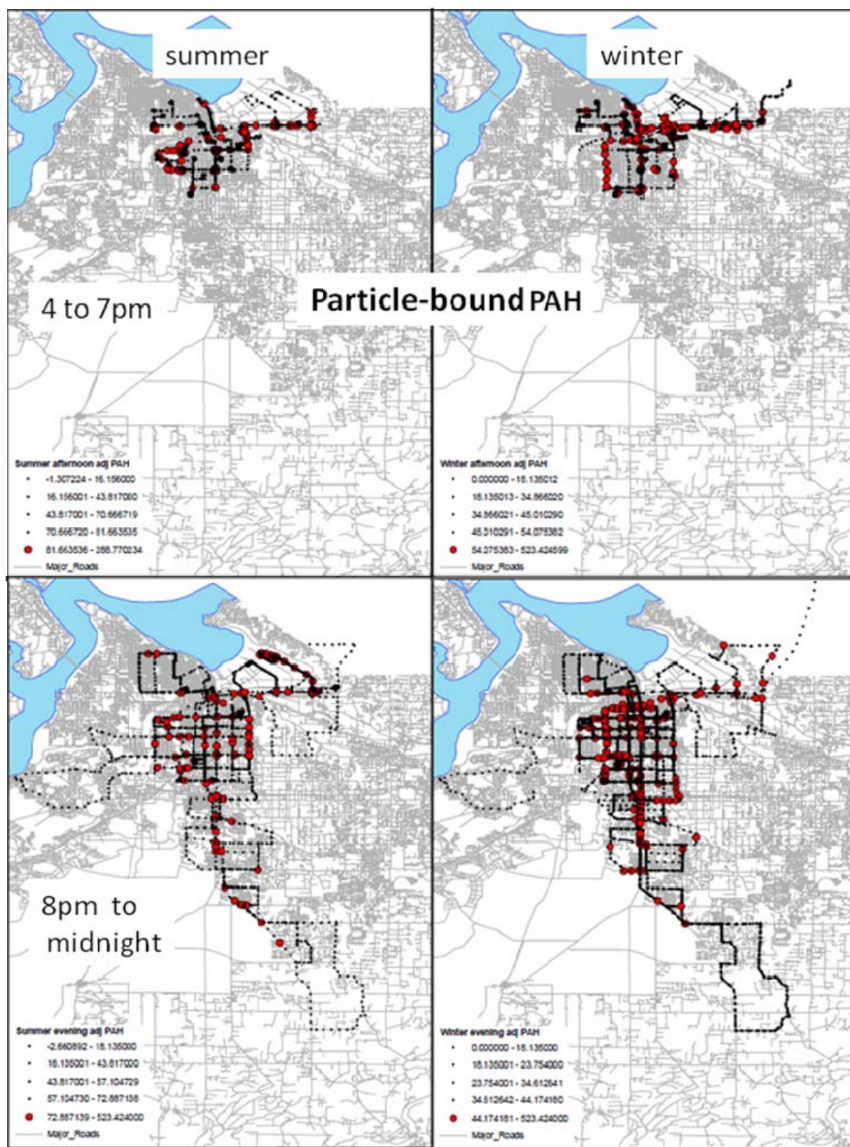
Figure 3.3.3: Spatial Distribution of Temporally Adjusted Particle-Bound PAHs (measurements were taken in the late afternoon and evening on selected winter days between December 2008 and February 2009 and on selected summer days between July and August 2009)
