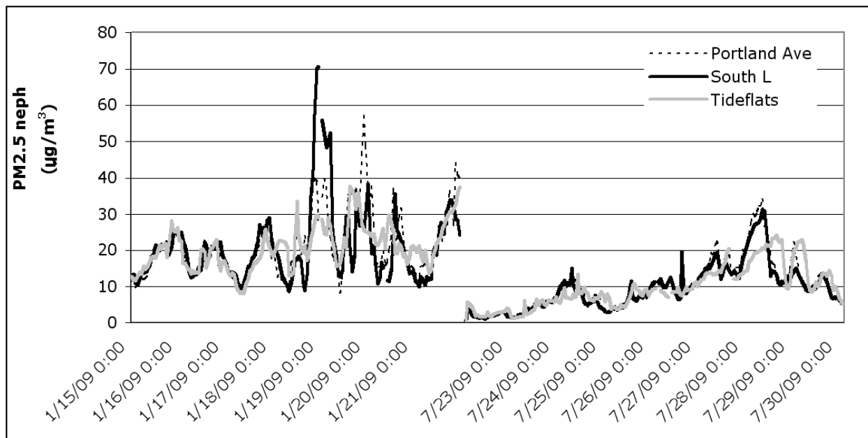
Figure 3.2.3: Hourly PM 2.5 Variation at the 3 "Central" Sites during the winter and summer monitoring periods
