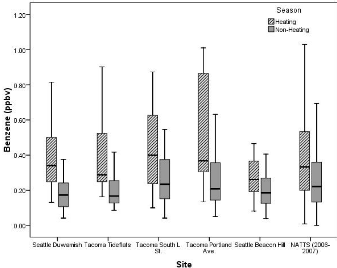
Figure 3.1.2: Box and Whisker Plots for Benzene: results by site and season
