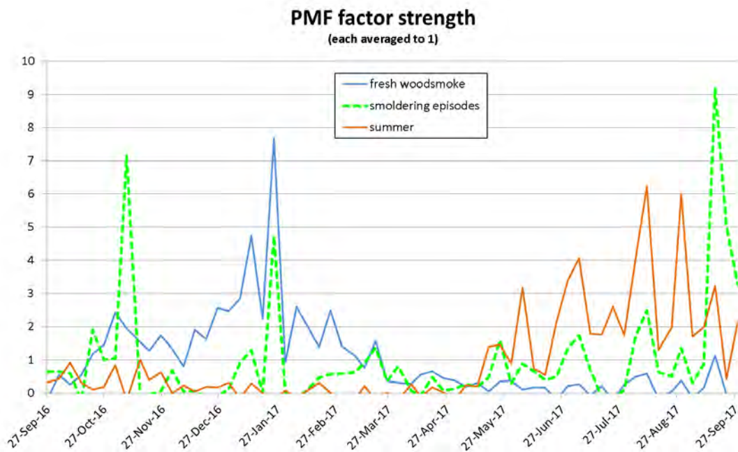
Figure 34. PMF factors 4-6 time series
