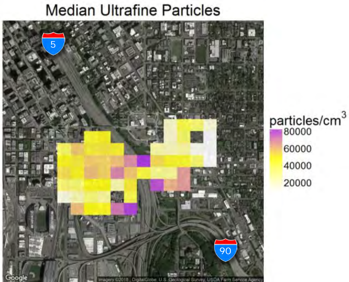
Figure 30. Map of median ultrafine particle counts.
