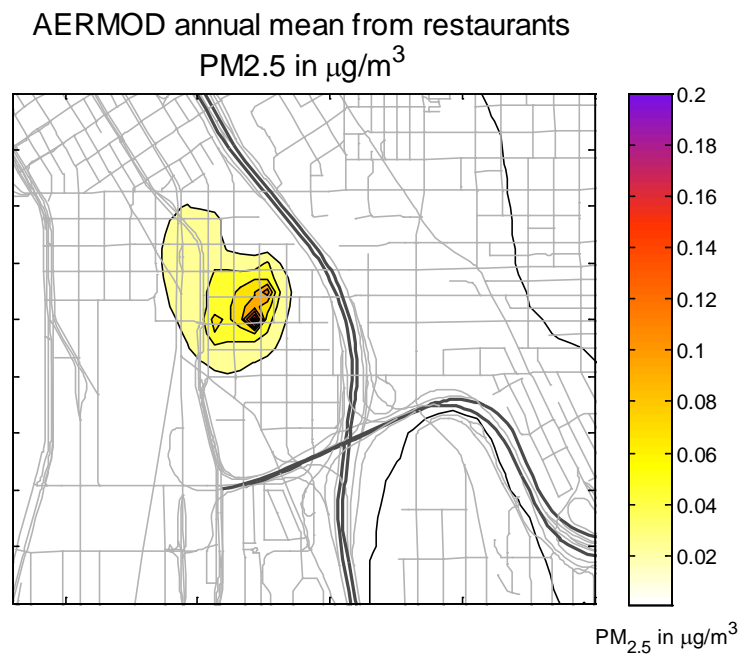
Figure 35. Modeled annual mean \text{PM}_{2.5} from restaurants.
