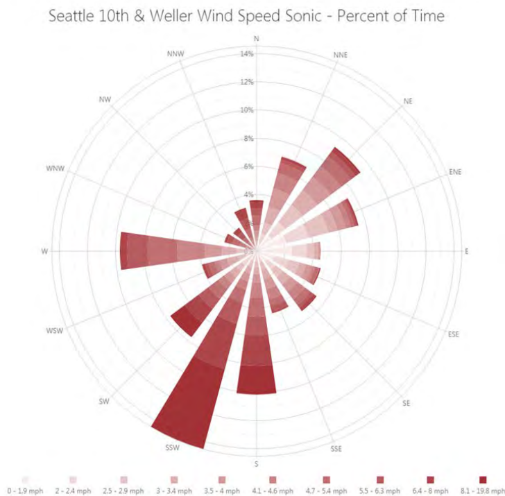
Figure 19. Wind rose at 10 th & Weller for the full campaign duration.
