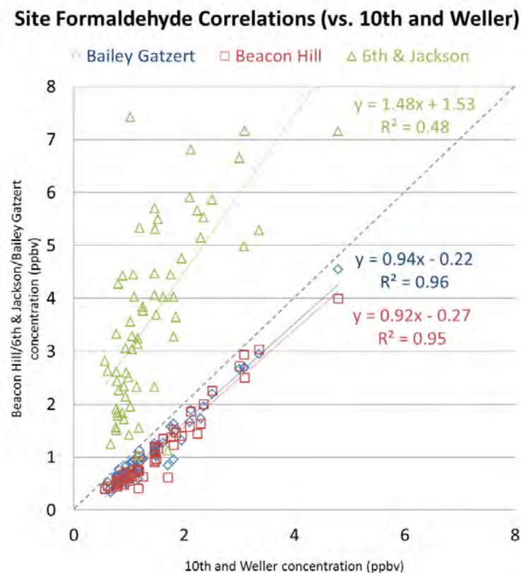
Figure 48. Site formaldehyde correlations with 10 th & Weller
