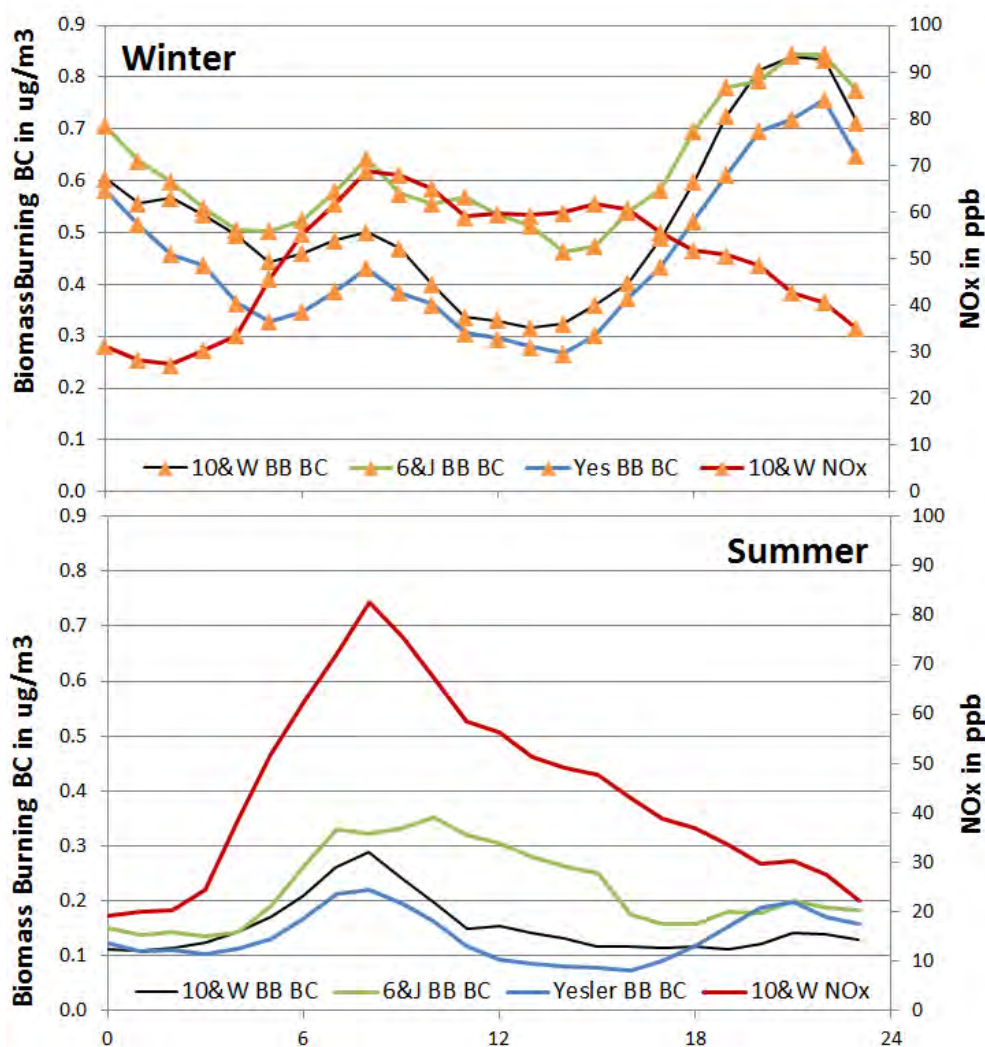
Figure 26. Diurnal pattern of biomass burning black carbon.
