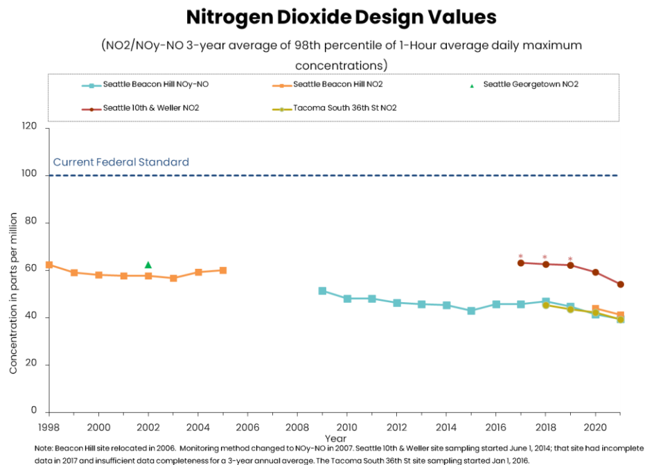
Figure 21: Nitrogen Dioxide (NO 2 ) (1998–2005) and Reactive Nitrogen (NO y – NO) (2007–2021) for the Puget Sound Region
